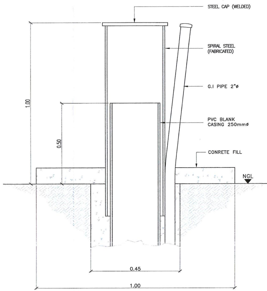
STEEL CASING DETAIL SCALE N T S
