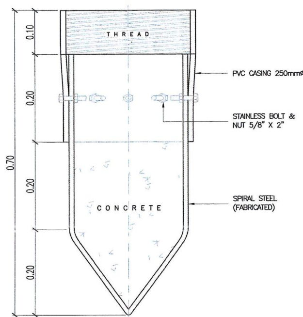
END CAP DETAIL SCALE N T S
