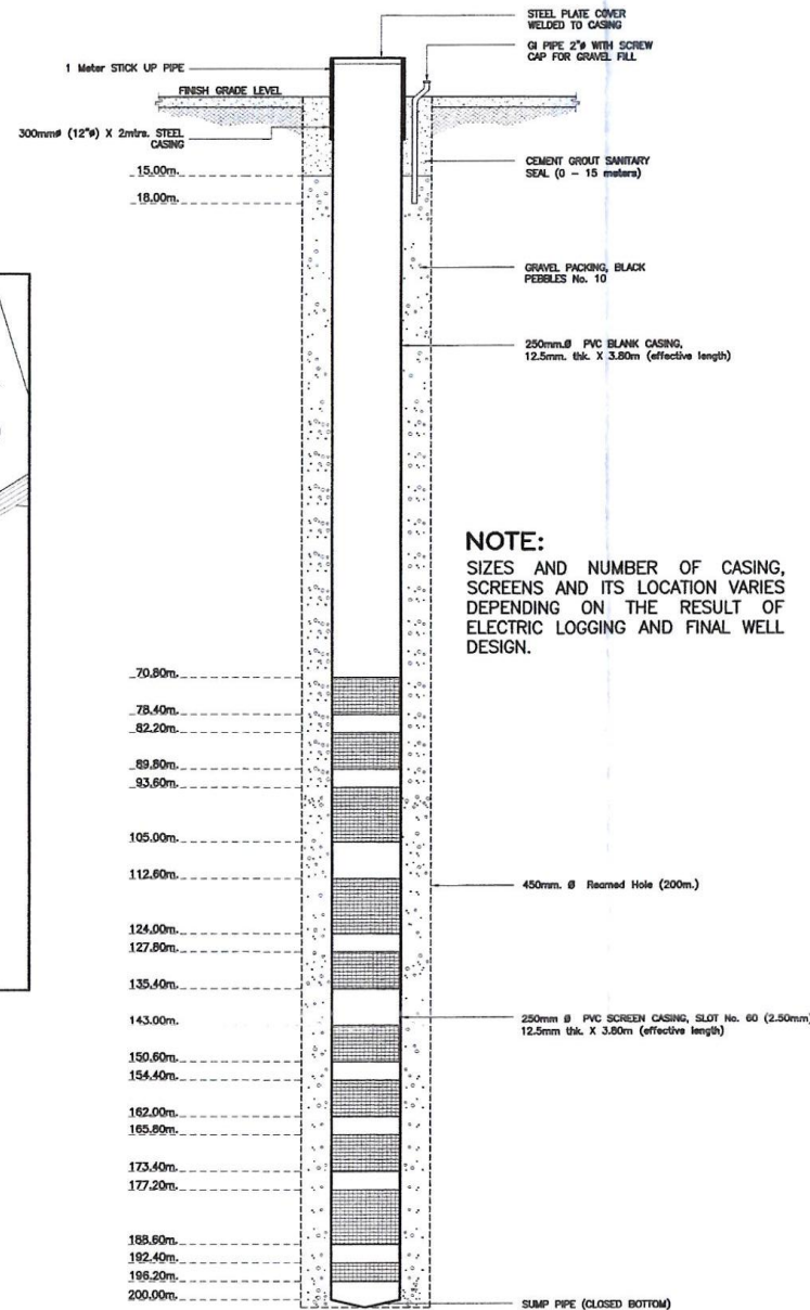
PRELIMINARY WELL DESIGN SCALE N T S
